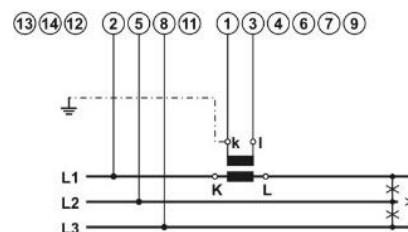
Three-phase – three-wire connection with balanced load
